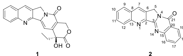
Figure 1. Structures of CPT ( 1 ) and luotonin A ( 2 ).
