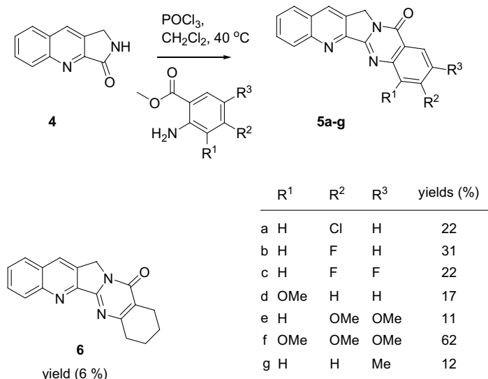
Figure 3. Synthesis of luotonin A derivatives 5a–g and 6 .
