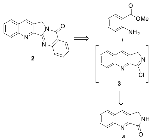
Figure 2. Retrosynthetic analysis of luotonin A.
