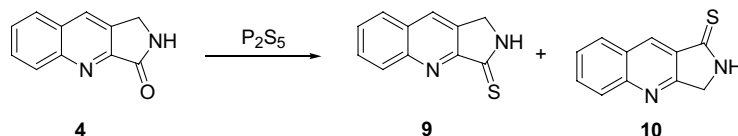
Figure 5. Synthesis of thiolactam 9 and formation of rearranged product 10 .
