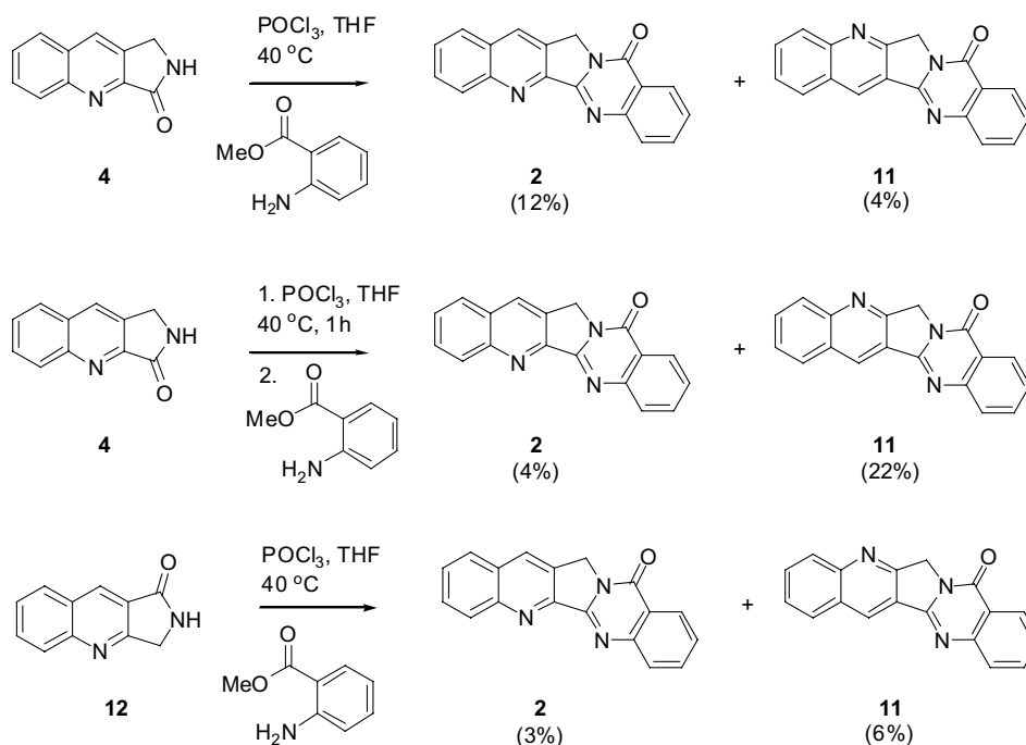
Figure 6. Synthesis of luotonin A ( 2 ) and formation of rearranged product isoluotonin A ( 11 ).
