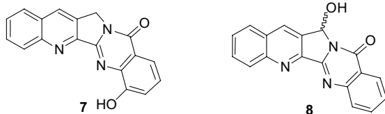
Figure 4. Structures of 16-hydroxyluotonin A (7) and luotonin B (8).
