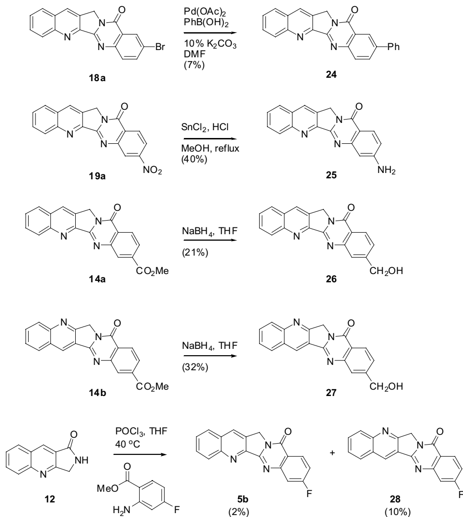
Figure 7. Conversion of luotonin A and isoluotonin A intermediates to new analogues.
