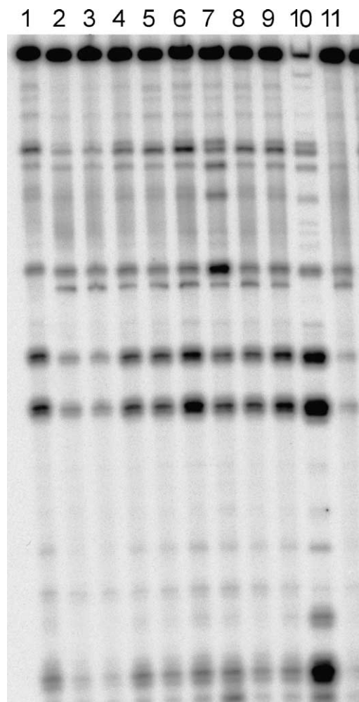
Figure 8. Autoradiogram of a 10% denaturing gel showing the effect of luotonin A analogues on human topoisomerase I-mediated cleavage of a 222-base pair DNA restriction fragment 3'- 32 P end labeled on the scissile strand. The individual incubation mixtures contained 36 ng of topoisomerase I and 50 \mu M luotonin A analogues as indicated. Following incubation at 37 °C for 30 min, the samples were digested with proteinase K prior to polyacrylamide gel analysis. Lanes 1–10, 50 \mu M compounds 11 , 17a , 17b , 22a , 22b , 25 , 26 , 28 , 2 , and 1 , respectively. Lane 11, DNA + topoisomerase I.
